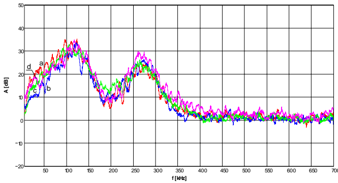
Fig. 2. Amplitude spectra of the AE signal generated by PDs for four electroinsulation oils of various physico-chemical parameters. a) oil No.1, b) oil No.2, c) oil No.3, d) oil No.4.
