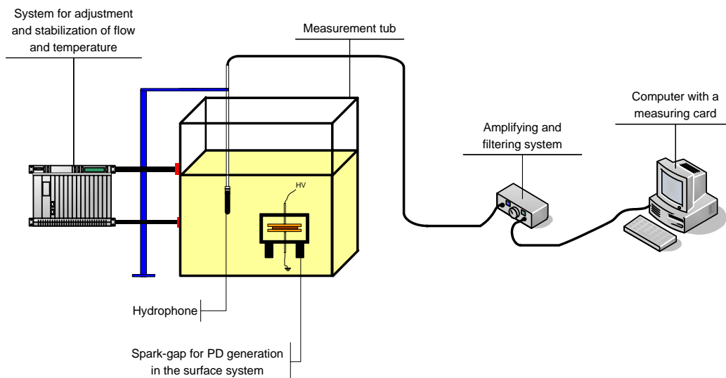
Fig. 1. Diagram of the measuring set-up for the measurement of the AE signals generated by PDs.
