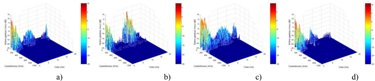
Fig. 4. Three-dimensional spectrograms of the spectrum density of energy determined for the AE signals generated by PDs in oils of various physico-chemical parameters.
