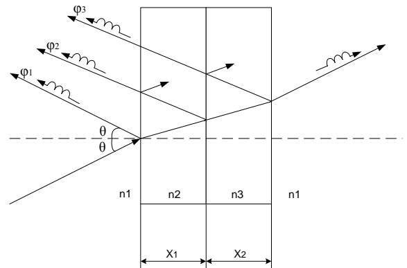
Fig. 1. The optical filter using two films.
