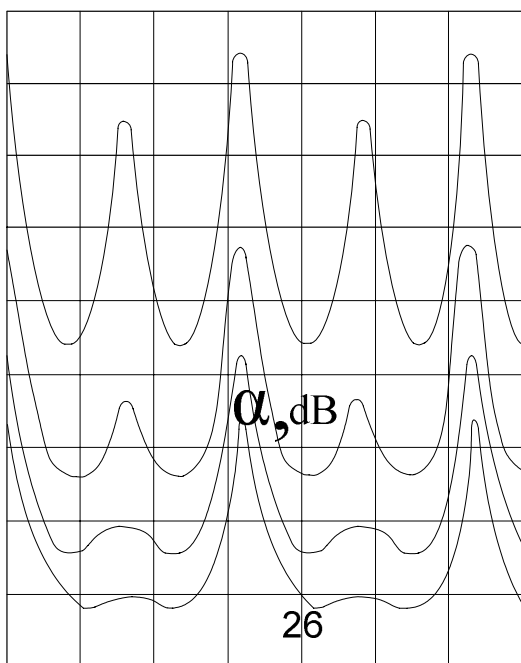
Fig. 2. Transmission filters response at n_2 = 1,8(1); 2,2(2); 2,5(3); 2,8(4) .
